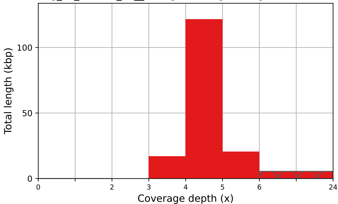
velvetg_on_dataset_98__Contigs coverage histogram (bin size: 1x)
